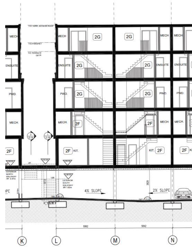
Cross-section
