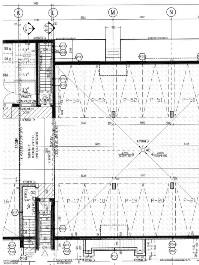
Garage Plan
