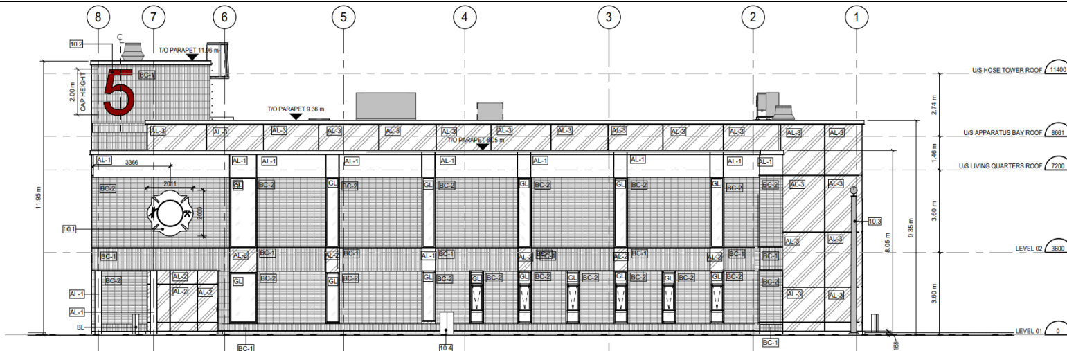
North Elevation (Flankage)
